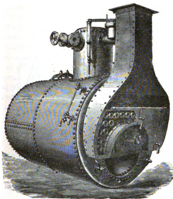
FIG. 34.—MARINE BOILER OF SMALL POWER.
